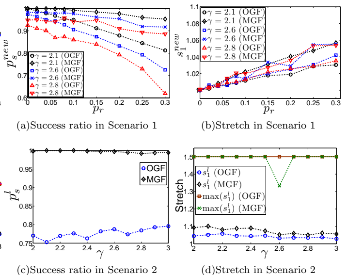
FIG. 10: (Color online) Greedy forwarding in dynamic networks.
