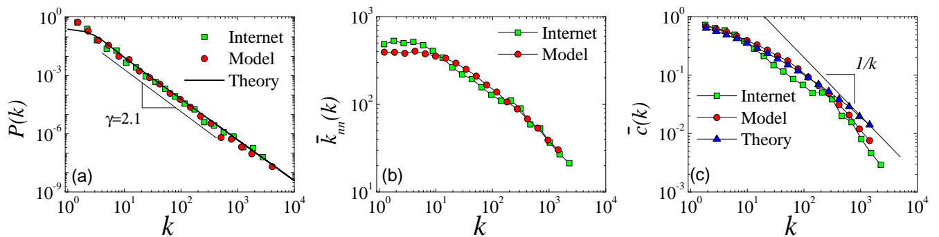
FIG. 8: (Color online) The Internet as seen by the CAIDA’s Archipelago Measurement Infrastructure [48] vs. a network in the \mathbb{H}^2 model with \alpha = 0.55 , \zeta = 1 , and \beta = 2 . (a) The degree distributions P(k) in both networks are power laws with exponent \gamma = 2.1 . The theoretical curve is given by (28). (b) The average nearest neighbor degrees \bar{k}_{nn}(k) . (c) The degree-dependent clustering. The theoretical curve is obtained by a numerical estimate of the outer integral in (59). The inner integral is \pi^2 \kappa' \kappa'' / (\kappa \kappa' + \kappa \kappa'' + \kappa' \kappa'') at \beta = 2 . The numerical integration is performed by summation over the node degrees k in the modeled network, i.e., \int d\kappa \rho(\kappa) \rightarrow \sum_k P(k) , and by mapping \kappa ’s to k ’s via \kappa = k\bar{k}/k . Random graphs capturing the three metrics in (a-c) reproduce also many other important structural properties of the Internet [49].
