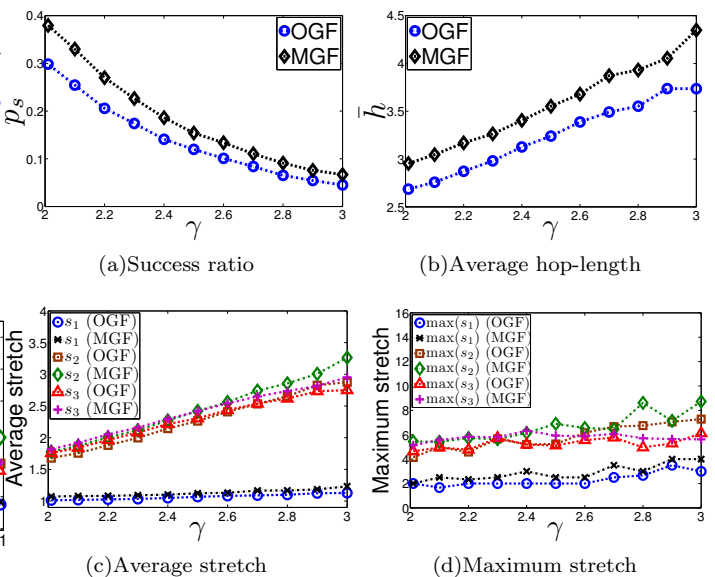
FIG. 12: (Color online) Greedy forwarding in the configuration model.
