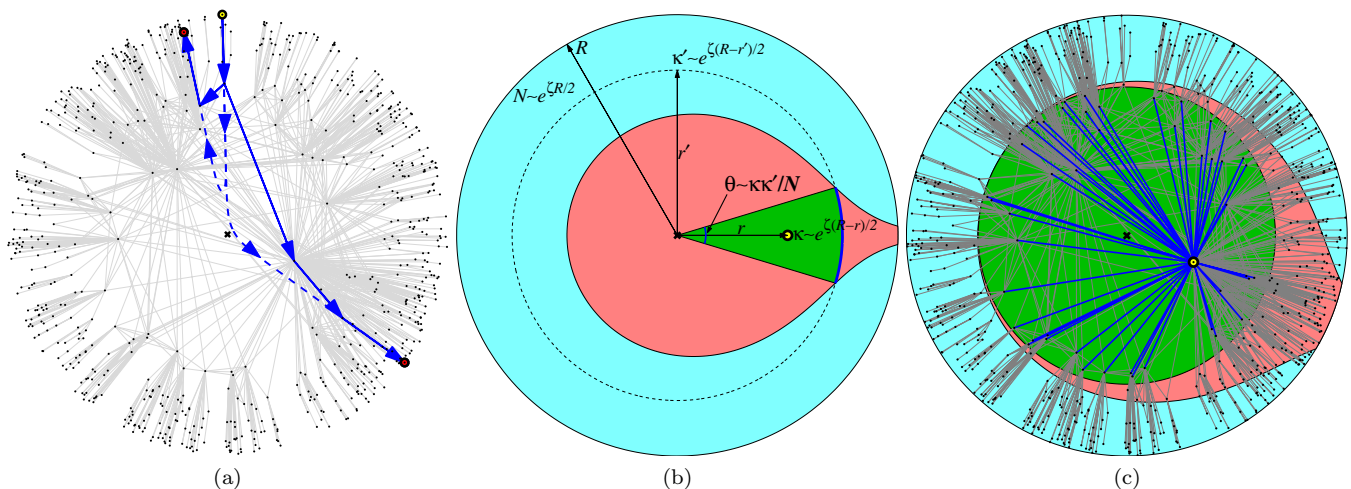
FIG. 13: (Color online) (a) Two greedy paths, which are also shortest paths ( s_1 = 1 ), from the source at the top to two destinations are shown by the solid arrows. The dashed curves are the hyperbolic geodesics between the same source and destinations. The hyperbolic stretches s_2 = s_3 of the left and right paths are 1.51 and 1.68. (b) The inner triangular shape (green) shows the angular sector \theta that the outer shape (red), which is the hyperbolic disk of radius R centered at the circled point located at distance r from the crossed origin, cuts out off the dashed circle of radius r' centered at the origin. The expected node degrees at r and r' are \kappa and \kappa' . (c) The circled node is an example of a bridge node. It is connected to all nodes in its hyperbolic disk of radius R (the outer shape (red)), including all nodes with expected degrees exceeding a certain threshold, or, equivalently, to all nodes with radial coordinates below a certain threshold, shown by the innermost disk (green) whose radius is R - r , where r is the radial coordinate of the circled node.
