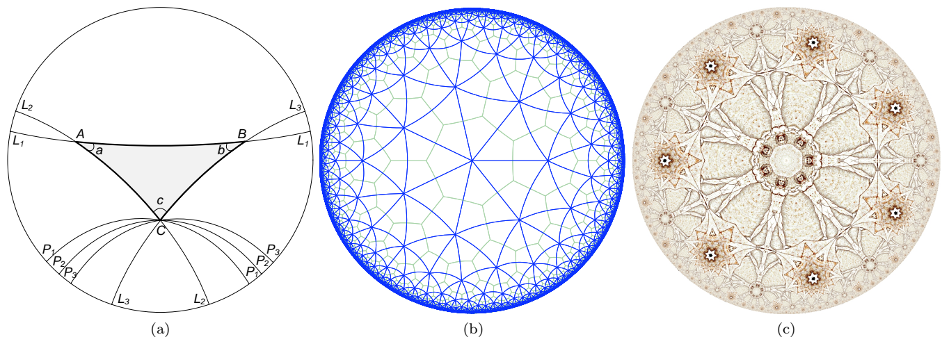
FIG. 1: (Color online) Poincaré disk model. In (a), L_{1,2,3} and P_{1,2,3} are examples of hyperbolic lines. Lines L_{1,2,3} intersect to form triangle ABC . The sum of its angles a + b + c < \pi . As opposed to Euclidean geometry, there are infinitely many lines (examples are P_{1,2,3} ) that are parallel to line L_1 and go through a point C that does not belong to L_1 . In (b), a \{7, 3\} -tessellation of the hyperbolic plane by equilateral triangles, and the dual \{3, 7\} -tessellation by regular heptagons are shown. All triangles and heptagons are of the same hyperbolic size but the size of their Euclidean representations exponentially decreases as a function of the distance from the center, while their number exponentially increases. In (c), the exponentially increasing number of men illustrates the exponential expansion of hyperbolic space. The Poincaré tool [1] is used to construct a \{7, 7\} -tessellation of the hyperbolic plane, rendering a fragment of The Vitruvian Man by Leonardo da Vinci.
