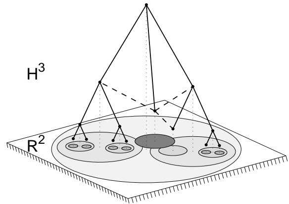
FIG. 2: Mapping between disks in the Euclidean plane \mathbb{R}^2 and points in the Poincaré half-space model of the three-dimensional hyperbolic space \mathbb{H}^3 [21]. The x, y -coordinates of disks in \mathbb{R}^2 are the x, y -coordinates of the corresponding points in \mathbb{H}^3 . The z -coordinates of these points in \mathbb{H}^3 are the radii of the corresponding disks. This mapping represents the tree-like hierarchy among the disks. Two points in \mathbb{H}^3 are connected by a solid link if one of the corresponding disks is the minimum-size disk that fully contains the other disk. This hierarchy is not perfect; thus, the tree structure is approximate. The darkest disk in the middle partially overlaps with three other disks at different levels of the hierarchy. Two points in \mathbb{H}^3 are connected by a dashed link if the corresponding disks partially overlap. These links add cycles to the tree. The shown structure is thus not strictly a tree, but it is hyperbolic [27].
