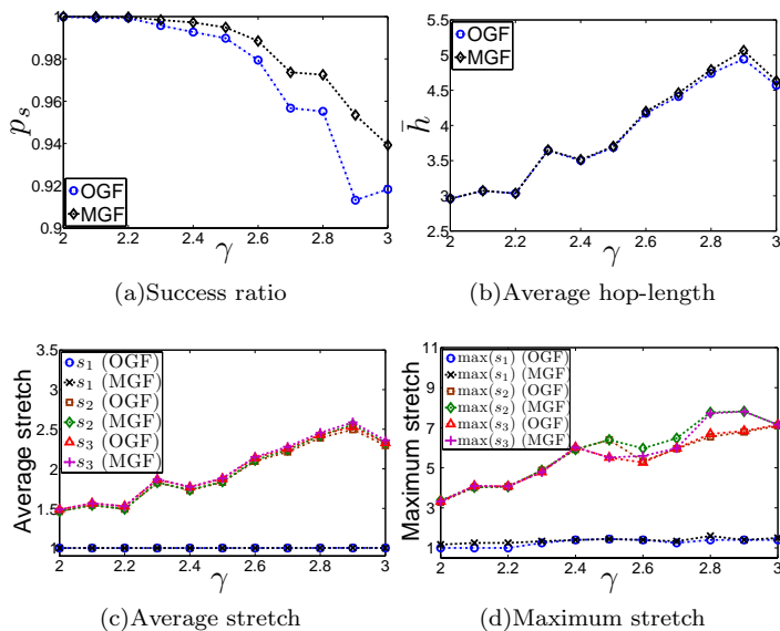
FIG. 9: (Color online) Greedy forwarding in static networks.
